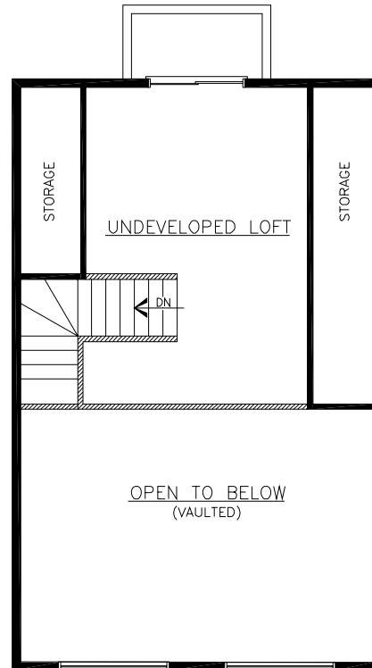
LOFT PLAN AREA = 209 S.F.
